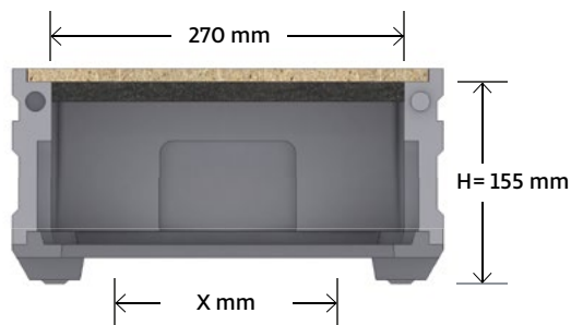
Image showing the maximum possible round cutout
